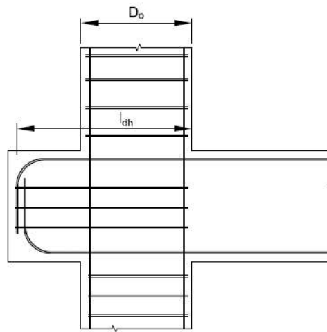
Figure 4-12 Provision of Beam stub
