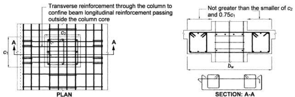
Figure 4-1 Maximum effective width of wide beam and required transverse reinforcement.
