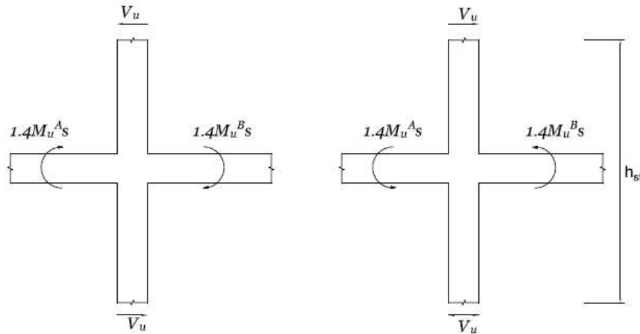
Figure 4-7 Calculation of Shear force demand in columns
