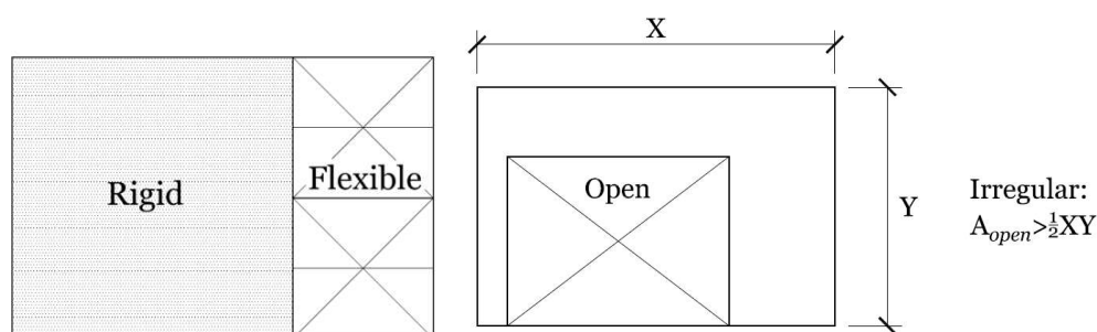
Figure 5-5: Diaphragm Discontinuity
