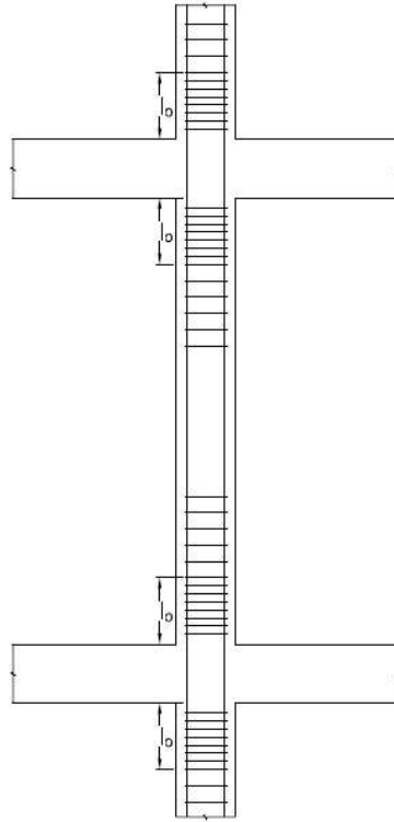
Figure 4-8 Confining stirrups in critical length l_o of column
