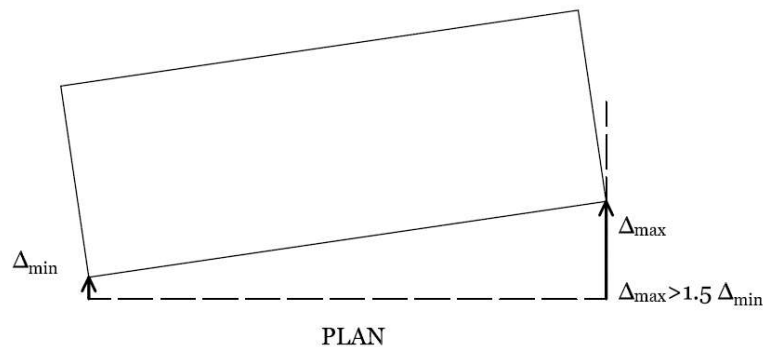
Figure 5-3: Torsion Irregularity
