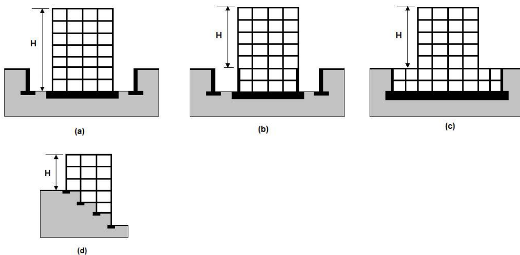
Figure 5-1: Height of Building
