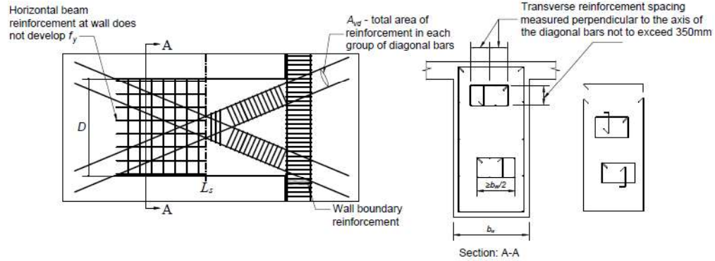
Figure 5-1 Coupling beams with diagonal reinforcement
