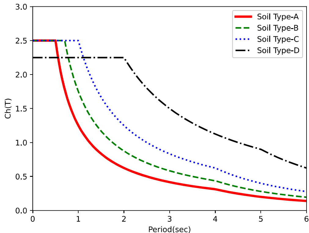
Figure 4-1 Spectral Shape Factor, C_h(T) for Equivalent Static Method
