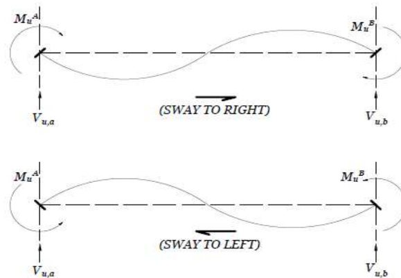
Figure 4-3 Calculation of Shear force demand in beams
