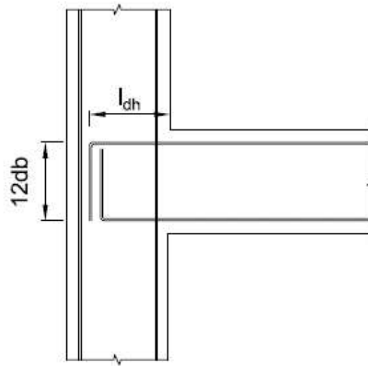
Figure 4-11 Anchorage of beam longitudinal bars in column
