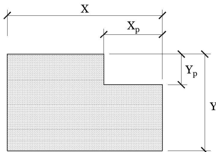
Figure 5-4: Re-entrant Corners
