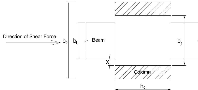
Figure 4-10 Effective joint width
