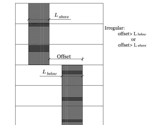
Figure 5-2: In-Plane Discontinuity
