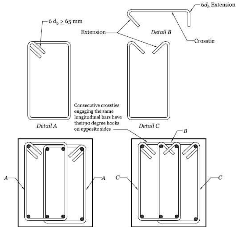
Figure 4-2 Details of Transverse reinforcement in beams
