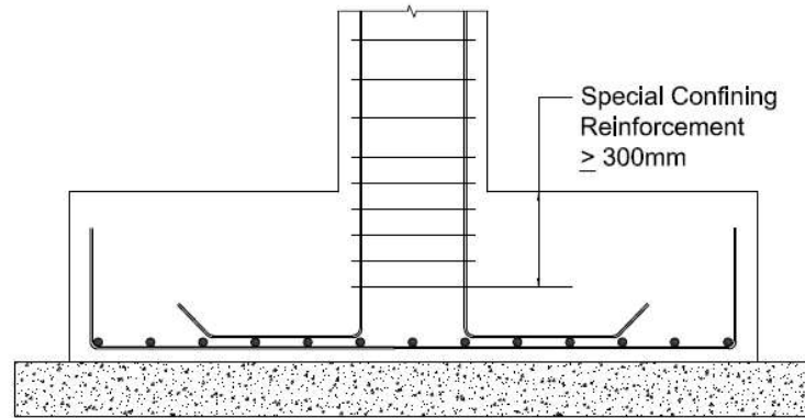
Figure 4-9 Confining reinforcement requirement in foundation
