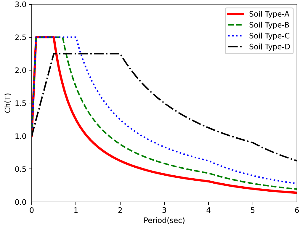
Figure 4-2 Spectral Shape Factor, C_h(T) for Modal Response Spectrum Method, Nonlinear Time History Analysis , Vertical Loading and Parts and Components
