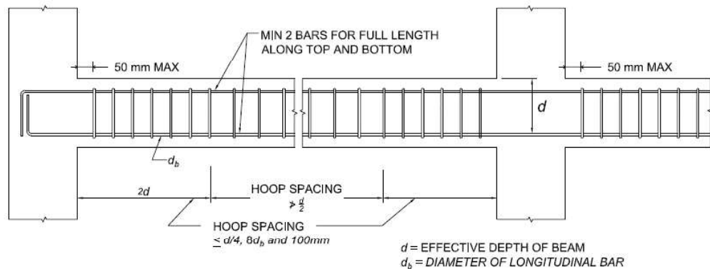
Figure 4-4 Details of transverse reinforcement in beams
