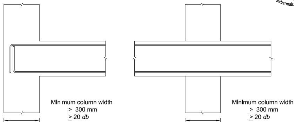
Figure 4-5 Requirement for minimum size of column member
